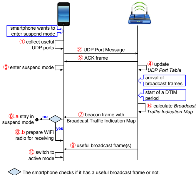
Figure 2. System Overview
