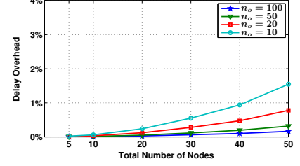
Figure 12. Increase in network delay with different numbers of UDP ports in use
