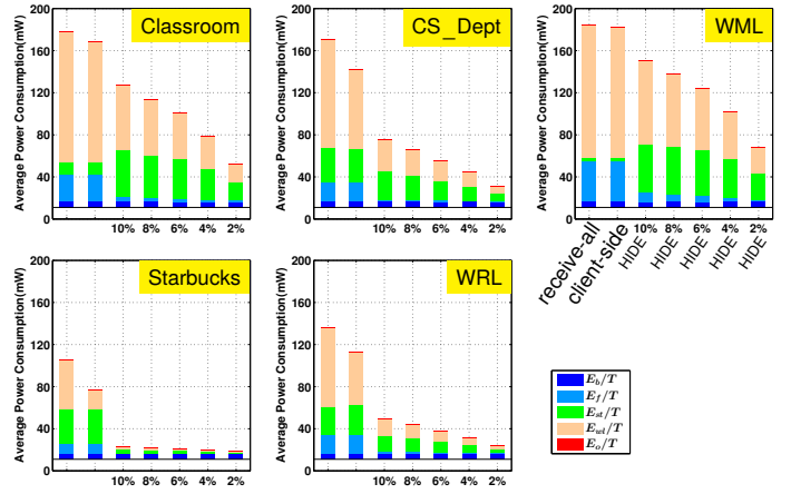
Figure 8. Energy consumption comparison (Galaxy S4). Numbers along x-axis are different percentages of useful broadcast frames.
