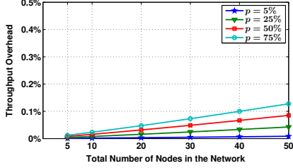
Figure 10. Decrease in network capacity with different percents of HIDE-enabled nodes
