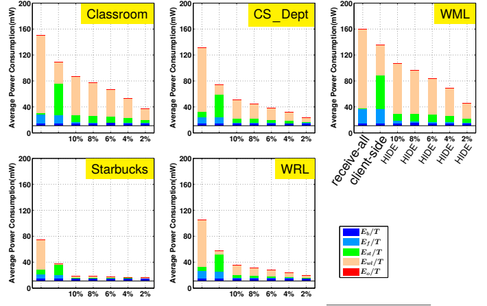
Figure 7. Energy consumption comparison (Nexus One). Numbers along x-axis are different percentages of useful broadcast frames.
