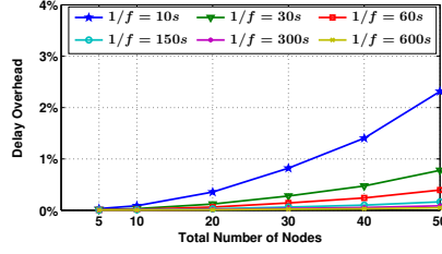
Figure 11. Increase in network delay with different sending intervals of UDP Port Messages
