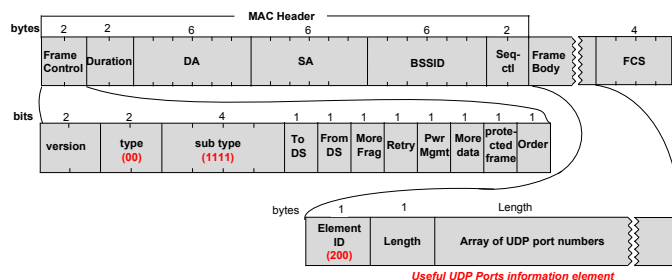
Figure 3. Frame structure of UDP port message
